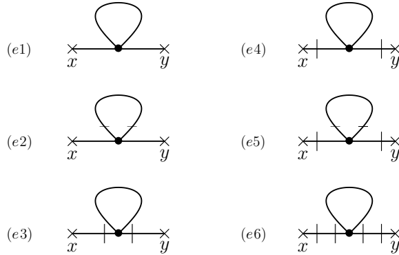
Figure 8. The six connected graphs contributing to the one-point Green’s function G_1 for the Hermitian theory to order g^3 . Graphs (e1), (e3) and (e4) are finite, but the remaining graphs are divergent and must be regulated.
