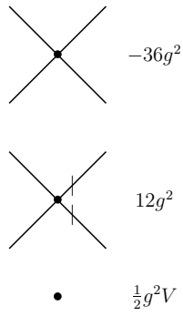
Figure 3. The three Euclidean-space vertices to order g^2 for the Hermitian Lagrangian \ell in (27). Note that the second vertex has tick marks on two of the legs. These tick marks indicate coordinate-space derivatives that arise because of derivative coupling. Derivative coupling results in divergent Feynman graphs.
