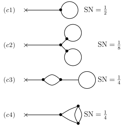
Figure 6. The Feynman graphs contributing to the one-point Green’s function G_1 of the non-Hermitian Hamiltonian H through order g^3 . Graph (c1) is of order g and graphs (c2)–(c4) are of order g^3 .
