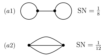
Figure 2. The two connected vacuum graphs, labelled (a1) and (a2), contributing to the ground-state energy of H in (18) to order g^2 . The symmetry numbers for each graph are indicated.
