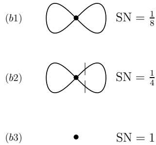
Figure 5. The three graphs contributing to the ground-state energy of the Hermitian Lagrangian \ell in (27) in order g^2 . Note that while graphs (b1) and (b3) are finite, the Feynman integral for graph (b2) diverges and must be regulated to obtain a finite result.
