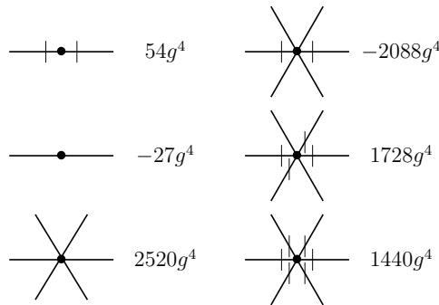
Figure 4. The six Euclidean-space vertices to order g^4 for the Hermitian Lagrangian \ell in (27). Note that four of the vertices have tick marks on the legs. These tick marks indicate derivative coupling.
