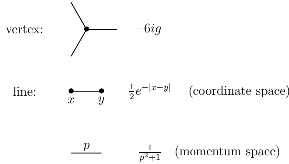
Figure 1. Feynman rules for the Lagrangian (23). For this simple local trilinear interaction the Feynman graphs are built from three-point vertices connected with lines. The line amplitudes in both coordinate space and momentum space are shown.
