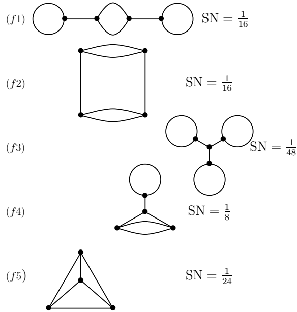
Figure 9. The five vacuum graphs contributing to the ground-state energy of the non-Hermitian \mathcal{PT} -symmetric Hamiltonian H in (18) to order g^4 . These graphs are all finite and very easy to evaluate.
