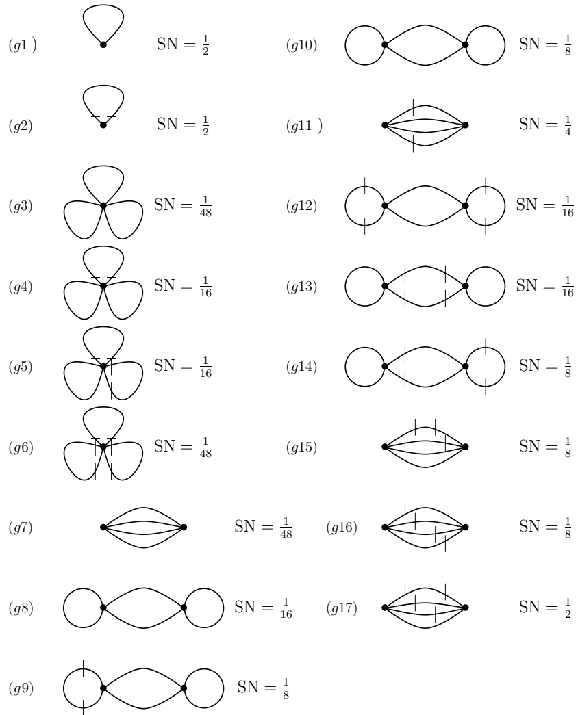
Figure 10. The 17 graphs contributing to the order g^4 term in the perturbation expansion for the ground-state energy of the Hermitian Hamiltonian h in (25). Note that ten of these graphs have divergent Feynman integrals. Of these ten, eight are relatively easy to regulate using dimensional continuation. However, graphs (g15) and (g17) have overlapping divergences and are therefore extremely hard to evaluate.
